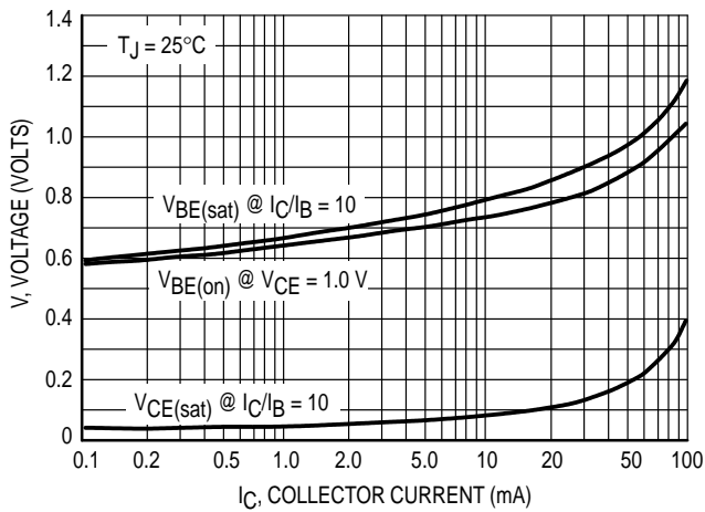
Figure 10. "On" Voltages
