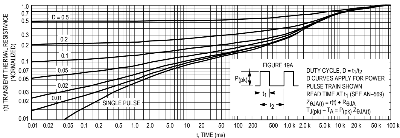
Figure 16. Thermal Response
